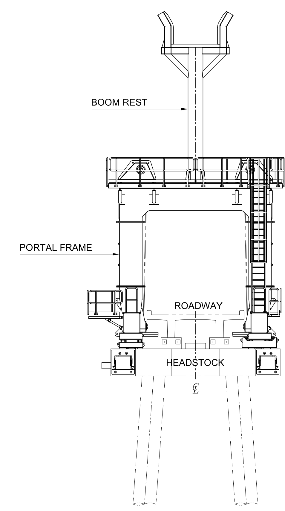
REAR VIEW SCALE 1:100
