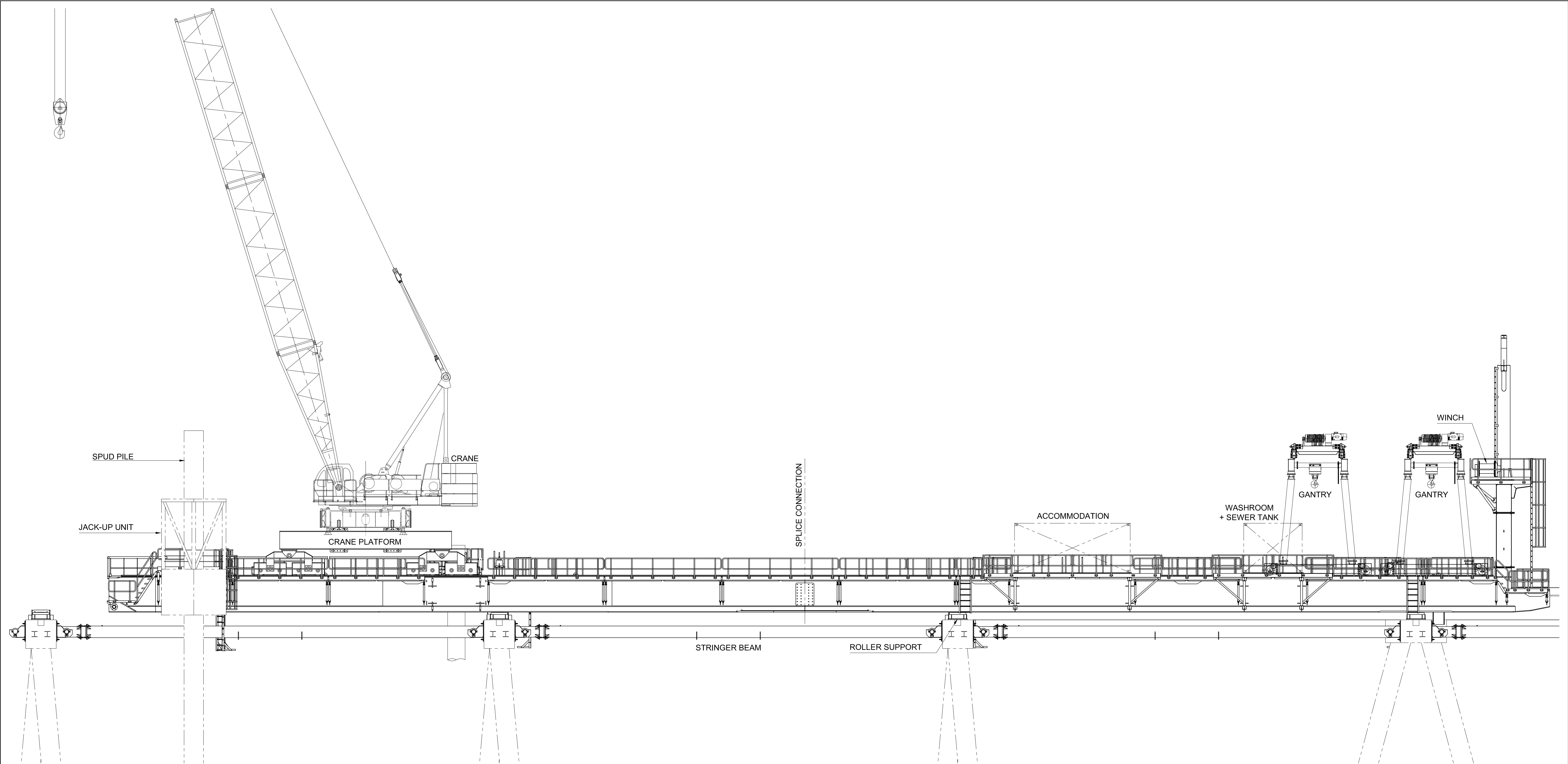
SIDE VIEW SCALE 1:100
